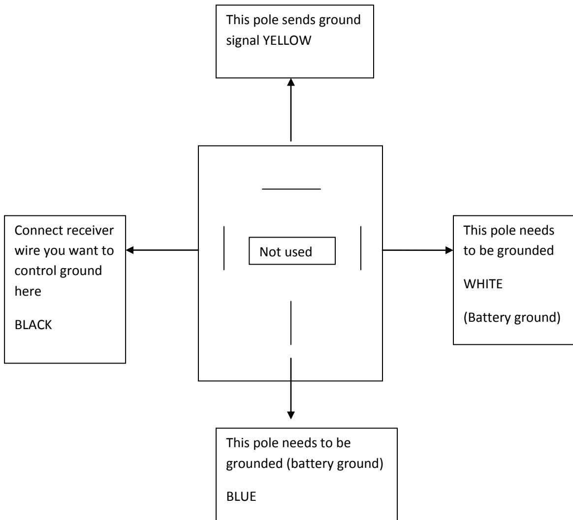
Grounding Diagram using a 30/40a automotive type relay
