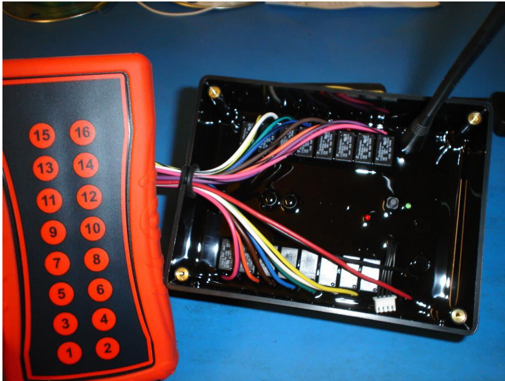
Fig. 1 Standard 16 Button Transmitter & Receiver Cover not shown
